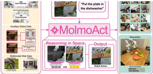
Figure 1 Overview. MolmoAct is an open action reasoning model that, given a user's language instruction, reasons in space and autoregressively predicts three structured reasoning chains: DEPTH PERCEPTION TOKENS for sensing and...
